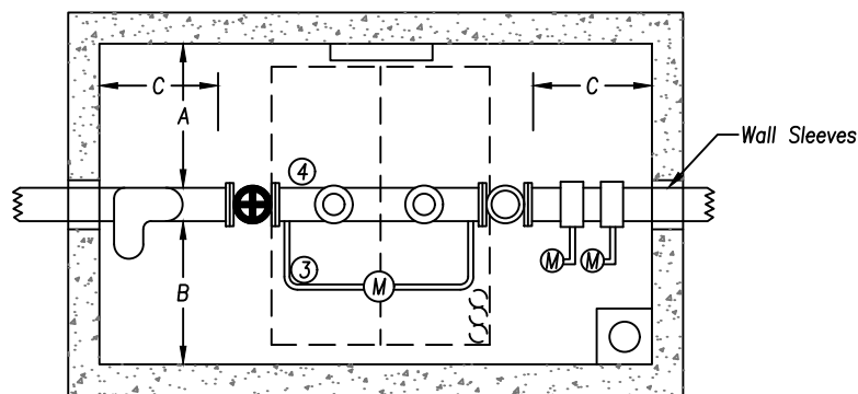
Precast pit to be approved by Director of Public Utilities
